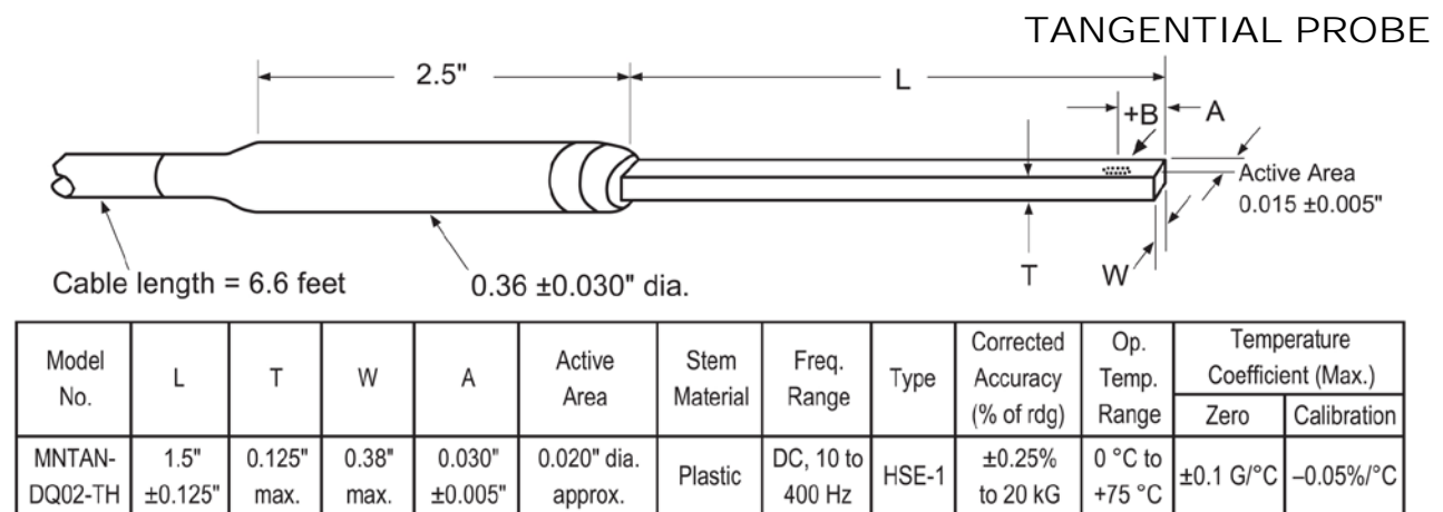
Figure 5-7. Definition of Lake Shore Tangential Probe
