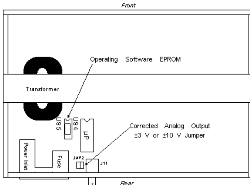
Figure 6-9. Location Of Operating Software EPROM
