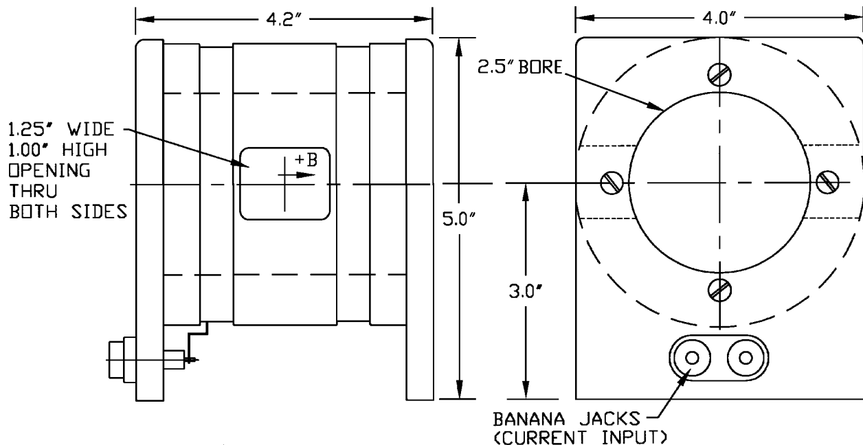
Figure 5-11. Model MH-2.5 Helmholtz Coil
