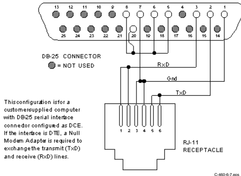
Figure 6-7. Model 4002 RJ-11 to DB-25 Adapter Wiring Details
