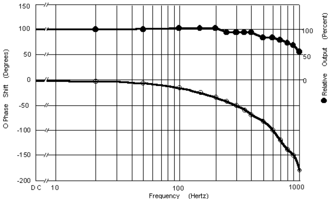
Figure 3-4. Monitor Analog Output Frequency Response
