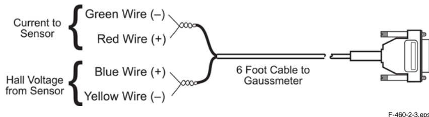
Figure 2-3. Model MCBL-XX User Programmable Cable Accessory
