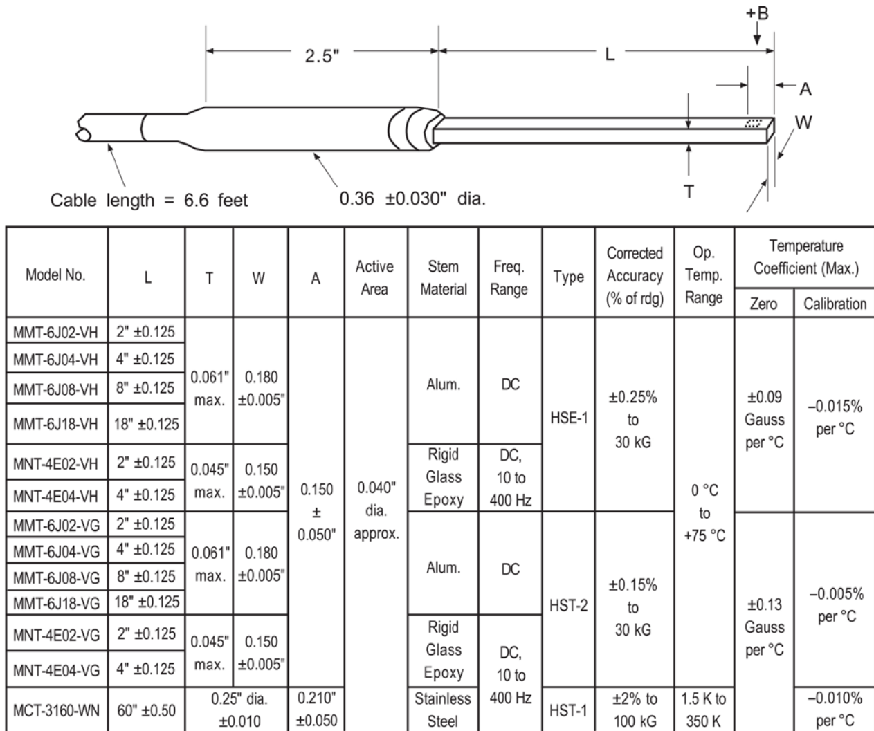
Figure 5-6. Definition of Lake Shore Transverse Probes
