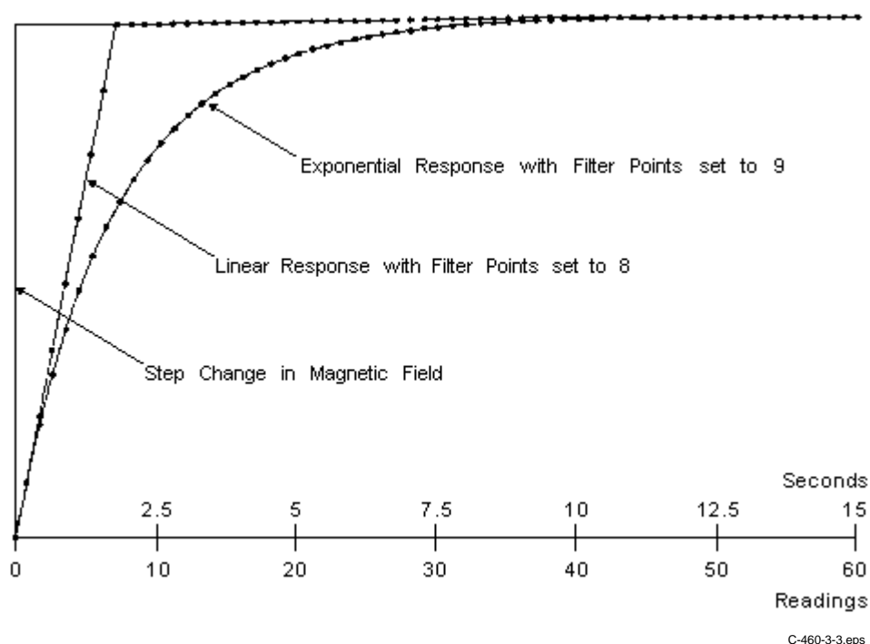
Figure 3-3. Display Filter Response Examples
