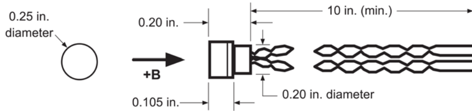
Figure C-5. Axial Hall Generator HGA-3010, HGA-3030, and HGCA-3020 Dimensions
