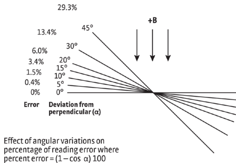
Figure 3-7. Effect Of Angle On Measurements
