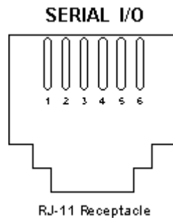
Figure 6-4. SERIAL I/O Connector Details
