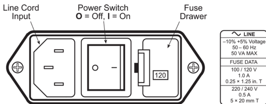
Figure 2-2. Line Input Assembly
