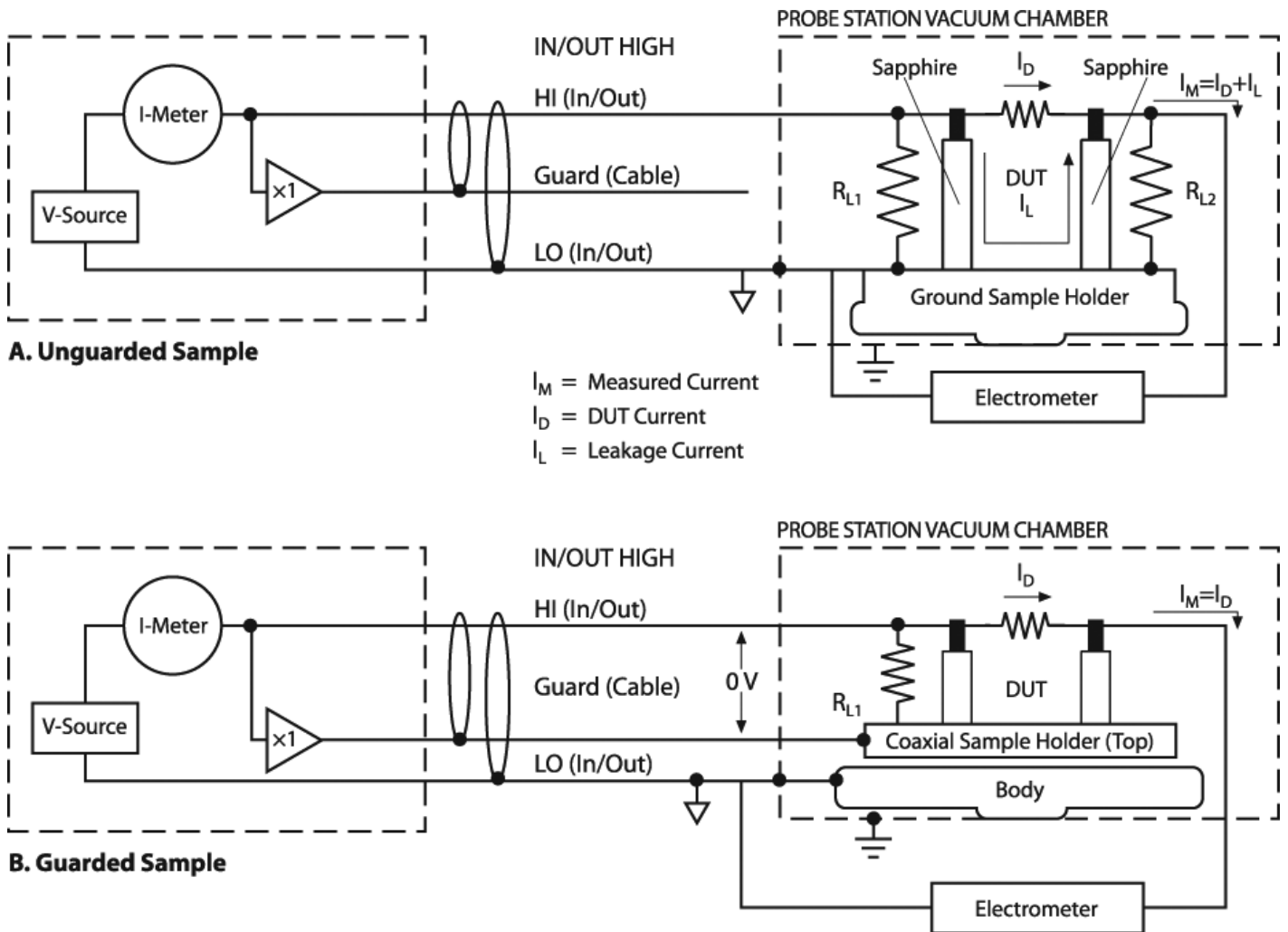
Figure 1 High impedance measurements
