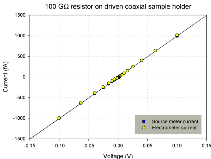
Figure 3 100 G \Omega resistor IV plot on driven coaxial sample holder
