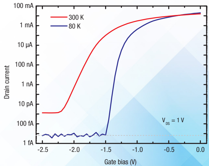
Figure 1 Temperature-dependent subthreshold characteristics of a silicon JFET.
