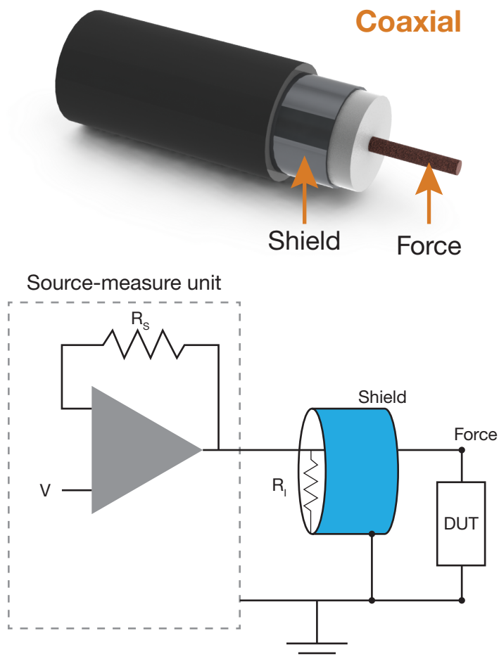
Figure 2 Conductors in a wire and device measurement layout using a coaxial configuration. Insulation leakage and charging effects in this configuration limit the low-current performance to roughly 1 nA.
