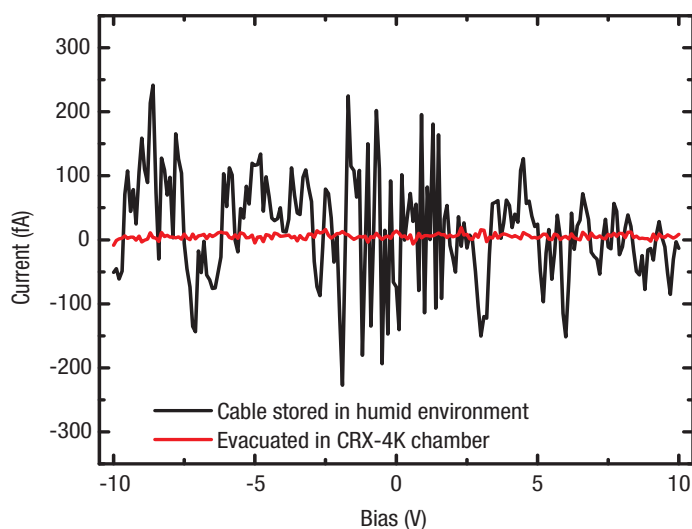
Figure 5. Leakage current for a vapor-saturated and evacuated triax feedthrough and cable. Electrochemical transport limits the current sensitivity of a device measurement and can be avoided by minimizing contamination of probing components as well as evacuating the sample space before each measurement.
