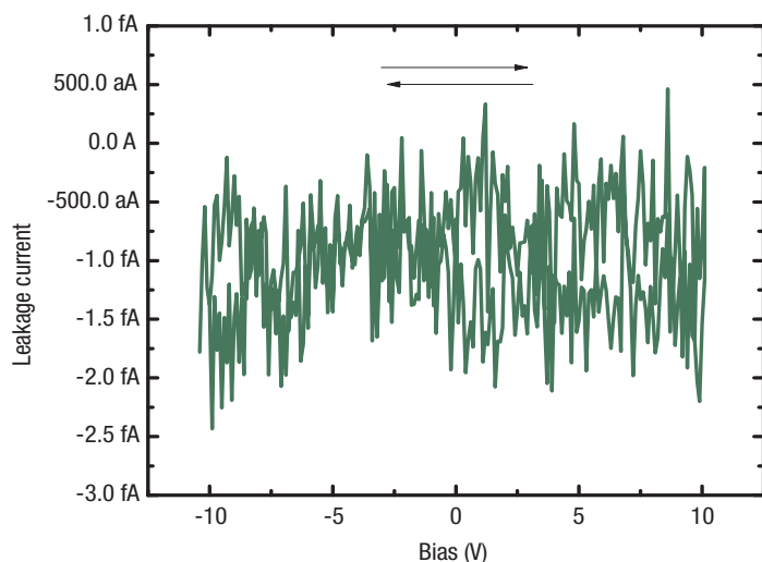
Figure 4 Measured leakage current in a Lake Shore triaxial probe arm assembly, including feedthrough, cable, and probe blade.
