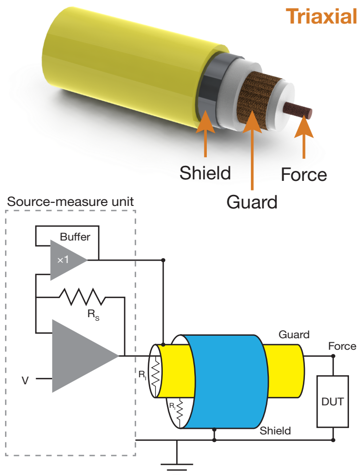
Figure 3. Conductors in a wire and device measurement layout using a triaxial configuration. The addition of a guard conductor reduces insulation leakage and charging effects in this configuration, leading to fA-scale low-current performance.
