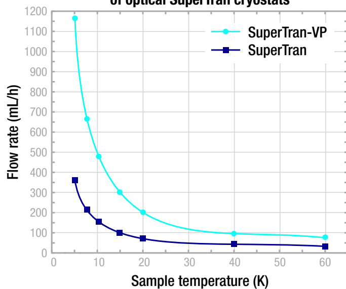
Typical cryogen consumption of optical SuperTran cryostats
