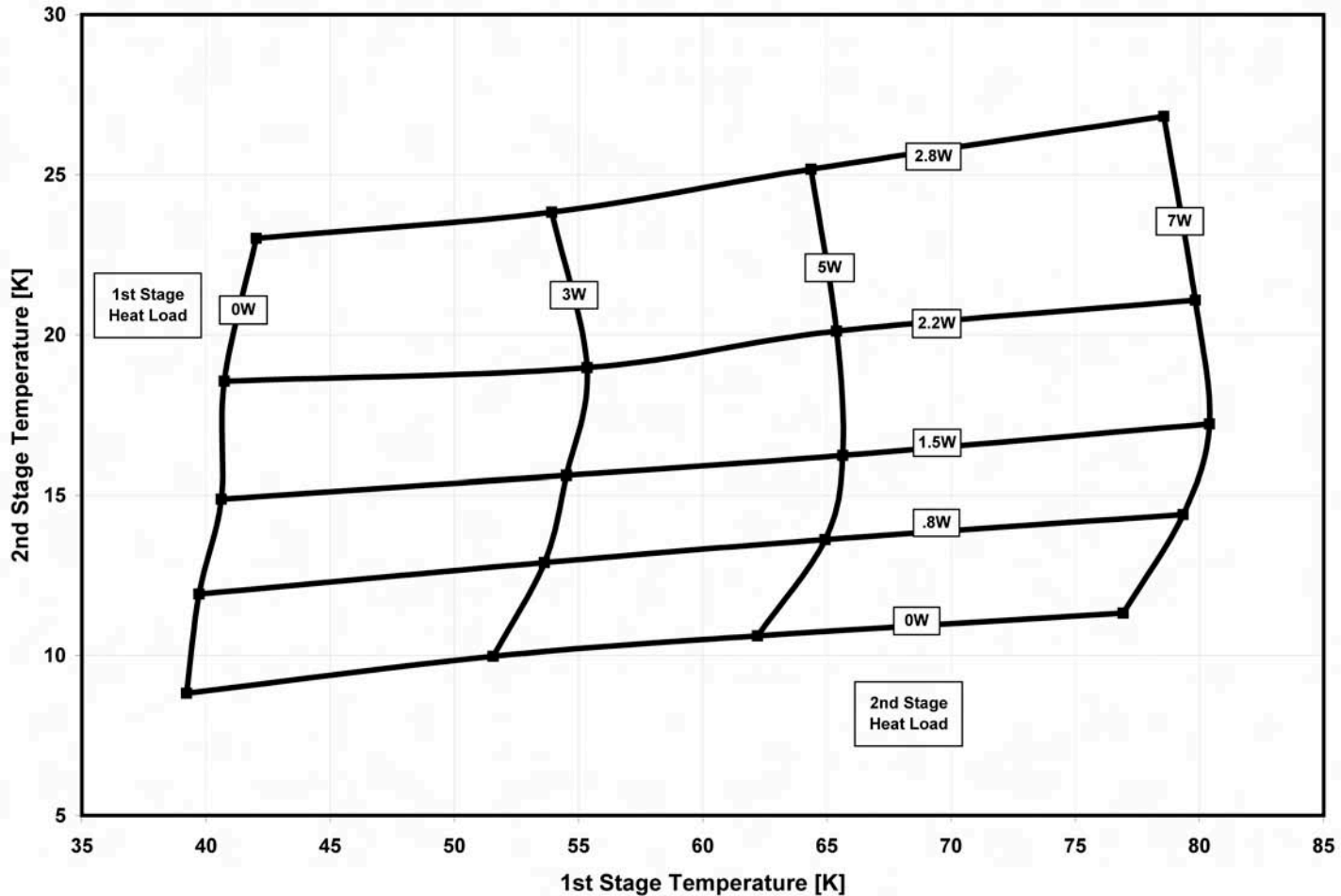
CH-202 Cold Head Capacity Map Using HC-4E1 Compressor at 50 Hz.
