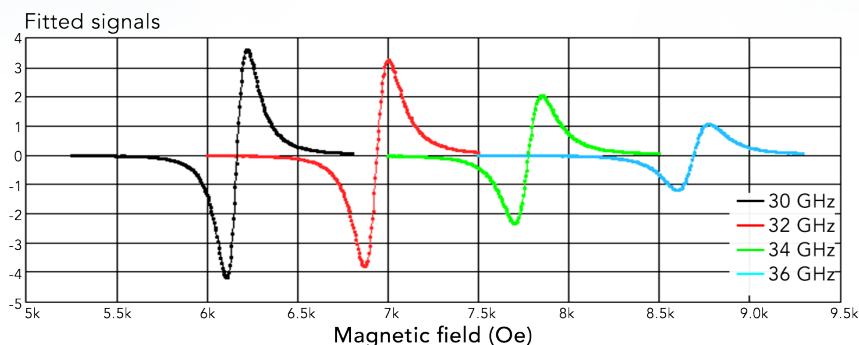
Measured and fitted data for \text{Ni}_{80}\text{Fe}_{20} (10 nm)/Ta (5 nm) thin film as a function of IP field to 0.94 T at frequencies of 30, 32, 34, and 36 GHz (typical results)
